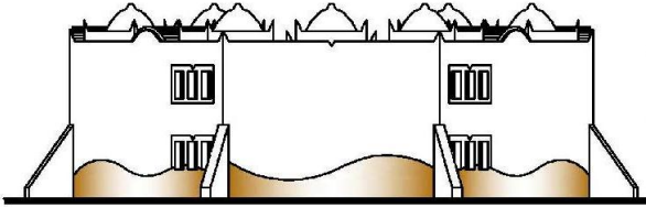
FACADE POSTERIEURE Echelle 1/100
