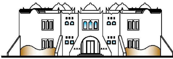
FACADE PRINCIPALE Echelle 1/100
